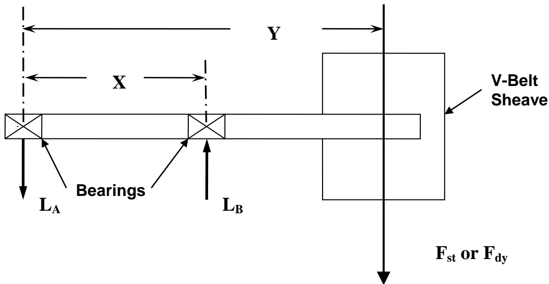
Figure #6: Cantilever Mount Belt Drive
