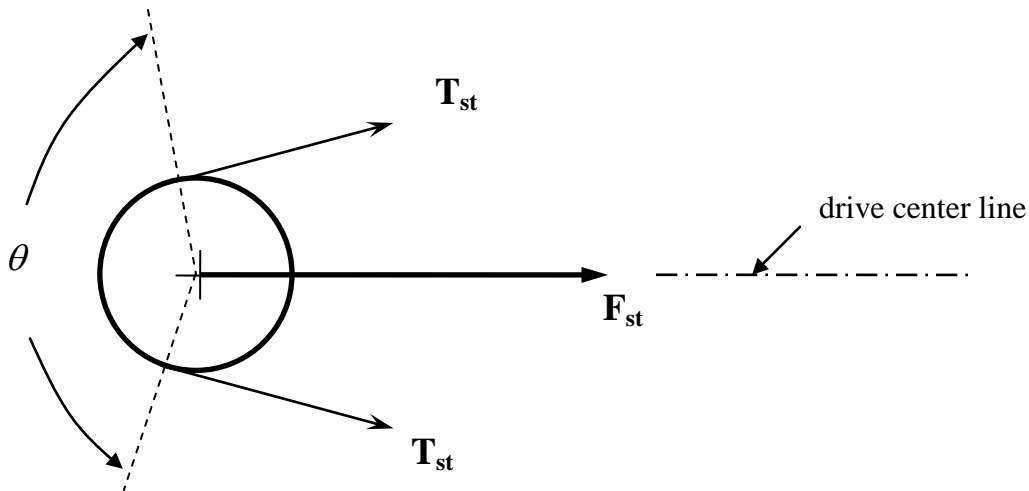
FIGURE #4: Static Shaft Load ( F_{st} )
