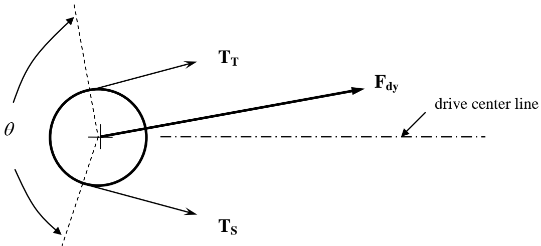
FIGURE #5 Dynamic Shaft Load ( F_{dy} )
