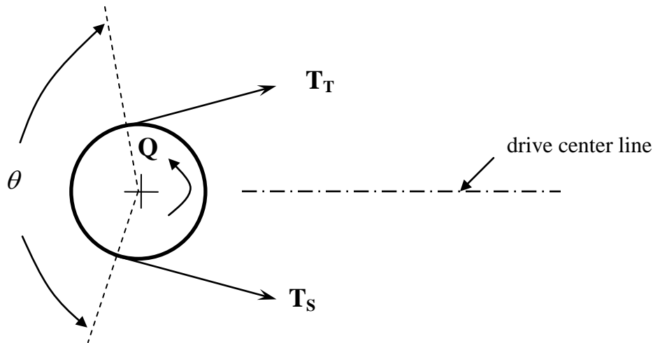
Figure #3: Belt Operating Tensions
